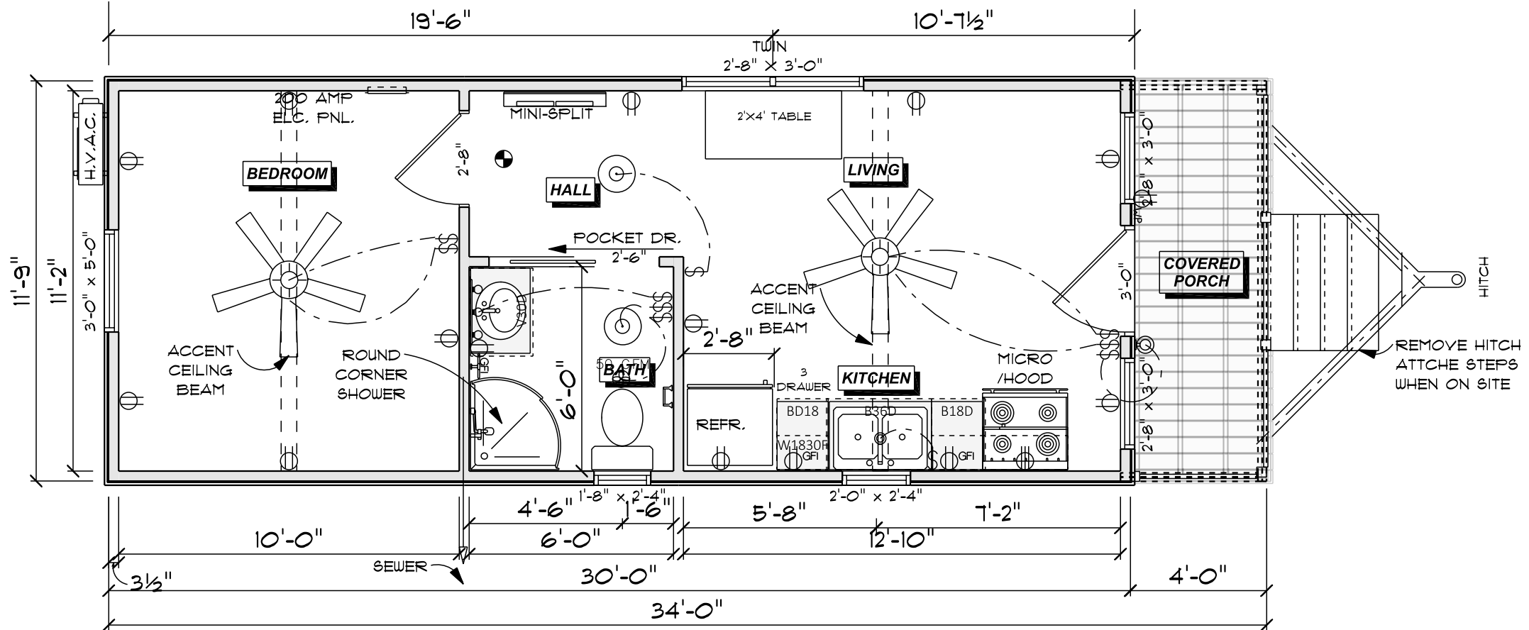
MAIN FLOOR SCALE: 1/4" = 1'-0"
