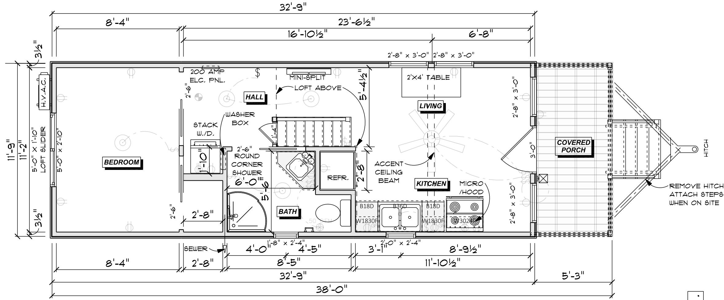
MAIN FLOOR SCALE: 1/4" = 1'-0"
