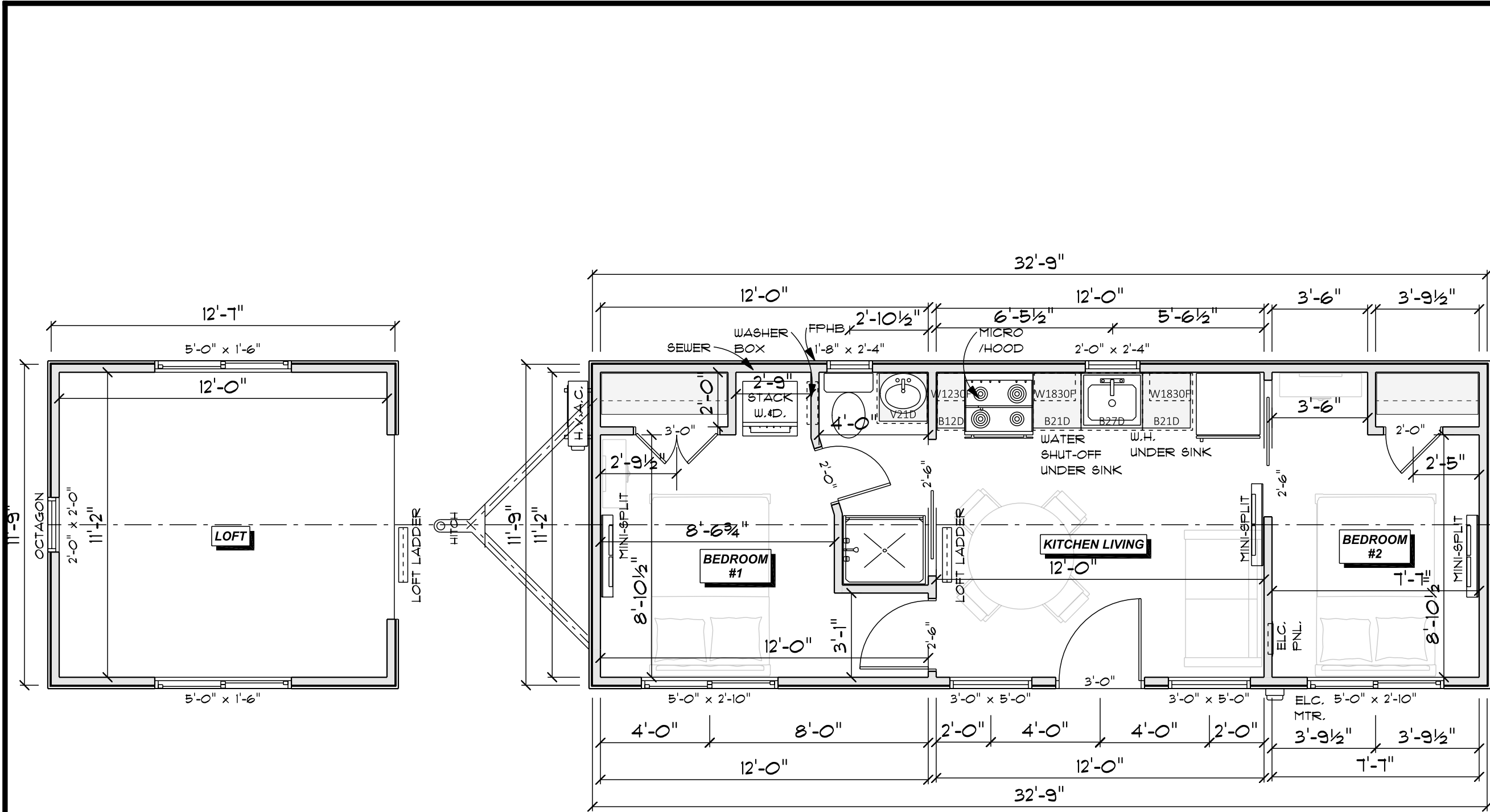
MAIN FLOOR SCALE: 1/4" = 1'-0"
